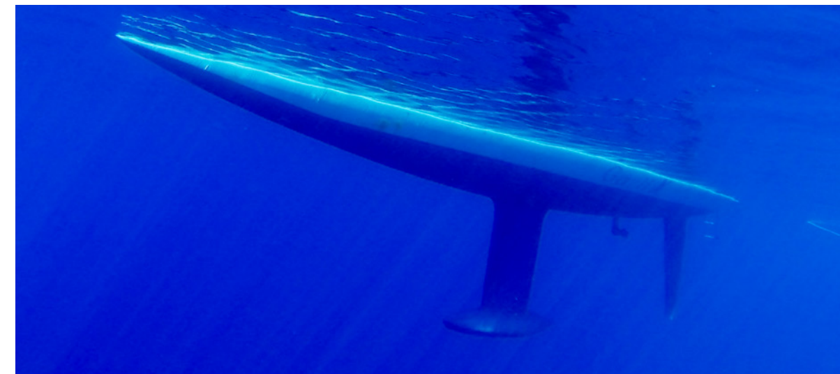
X-Yachts engine struts are faired into the hull for reduced drag and improved reliability
