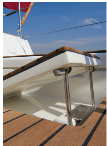
Adjustable folding foot chocks
